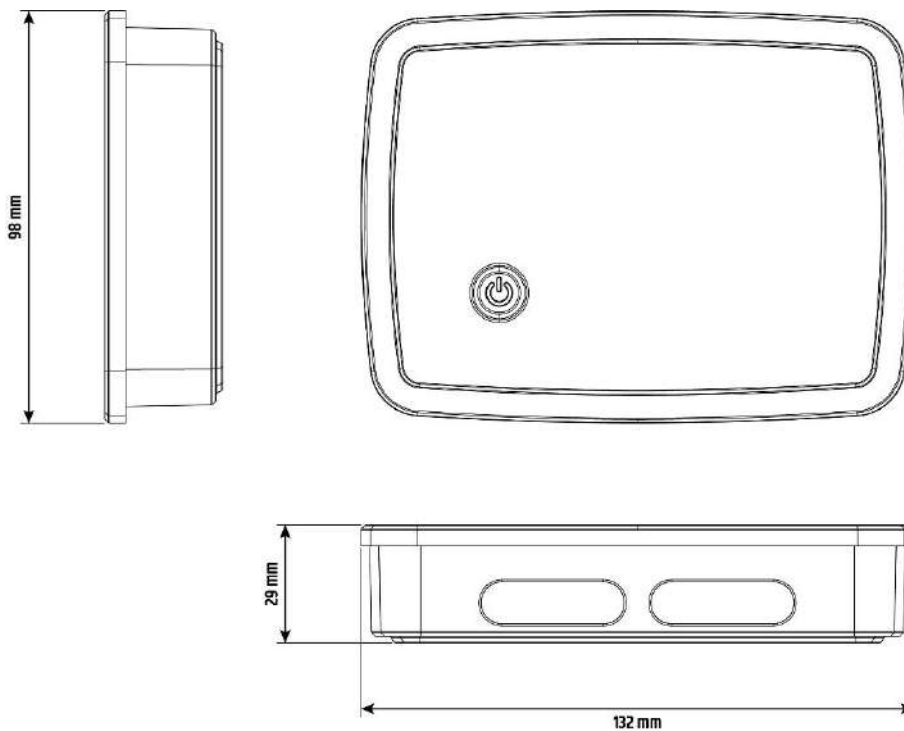
Device dimension.
